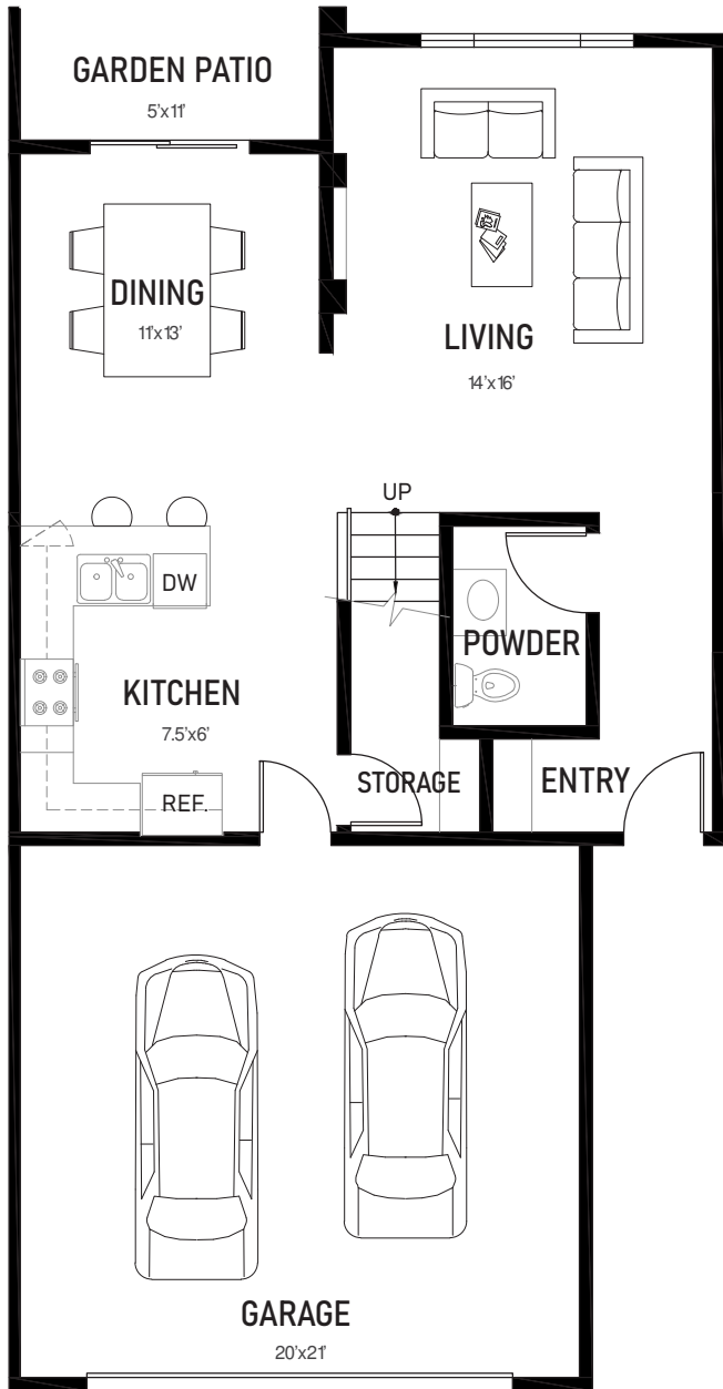
FIRST FLOOR
